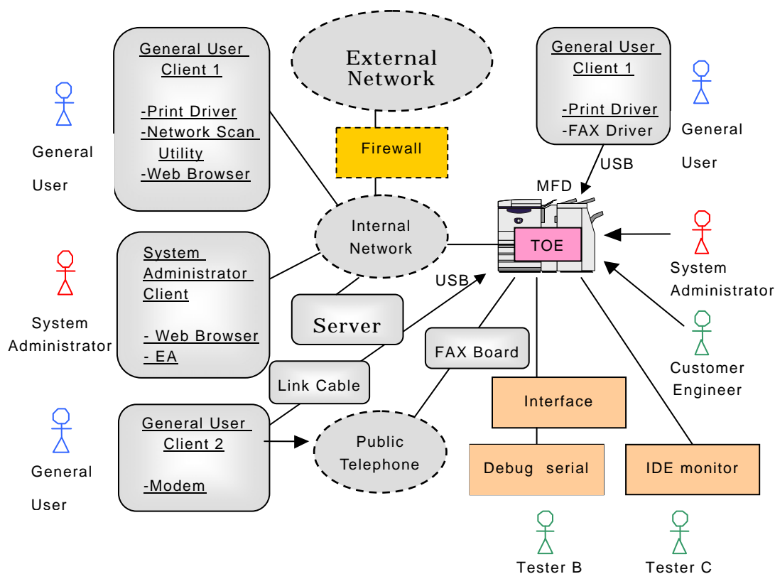
Figure 3-1 Configuration of Developer Testing
