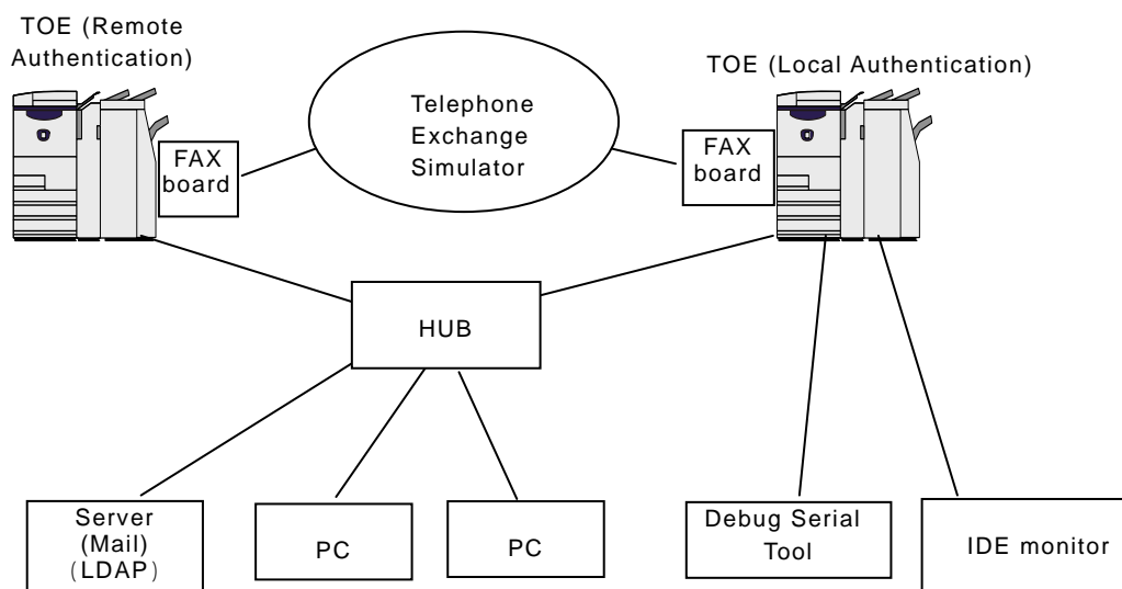
Figure 3-2 Evaluator Testing Configuration
