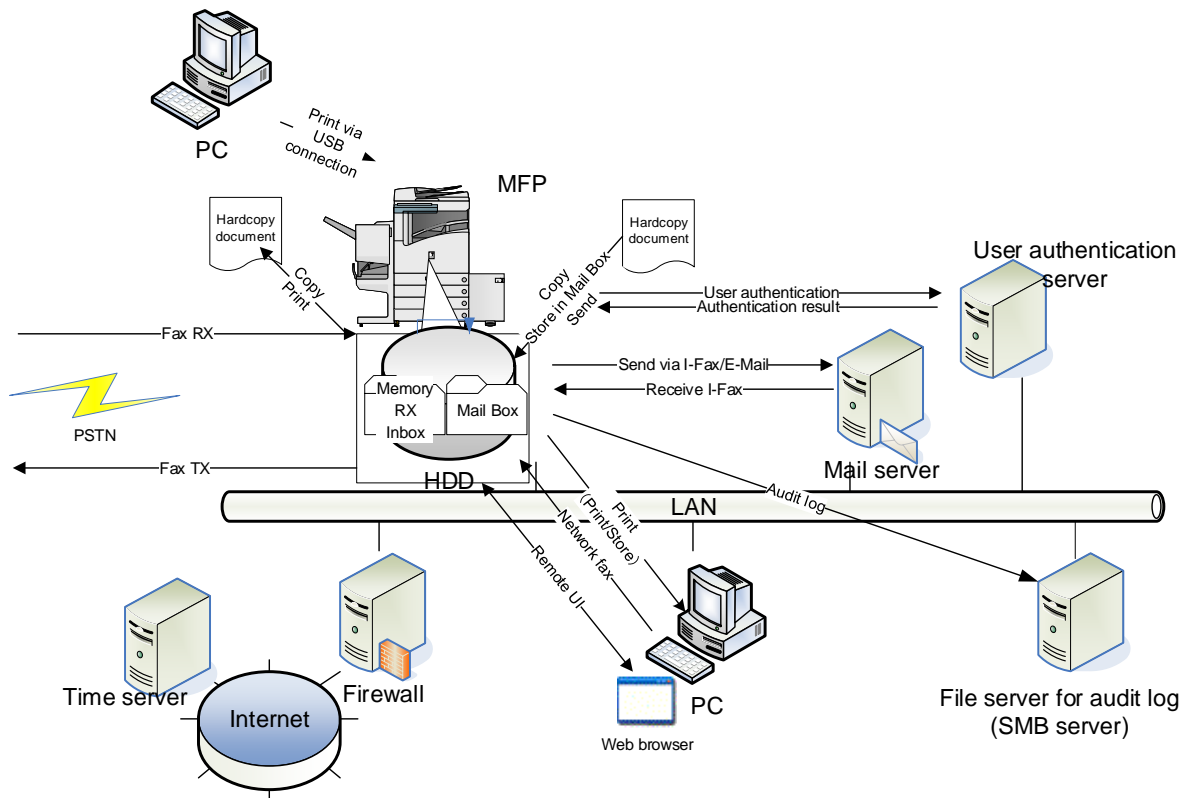
Figure 1 The assumed operational environment of the MFP < Canon imageRUNNER ADVANCE C356/C256 Series >
