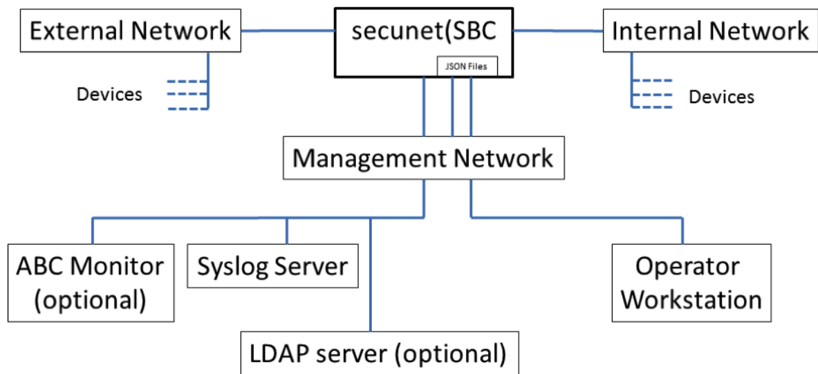
Figure 1 secunet SBC network topology
