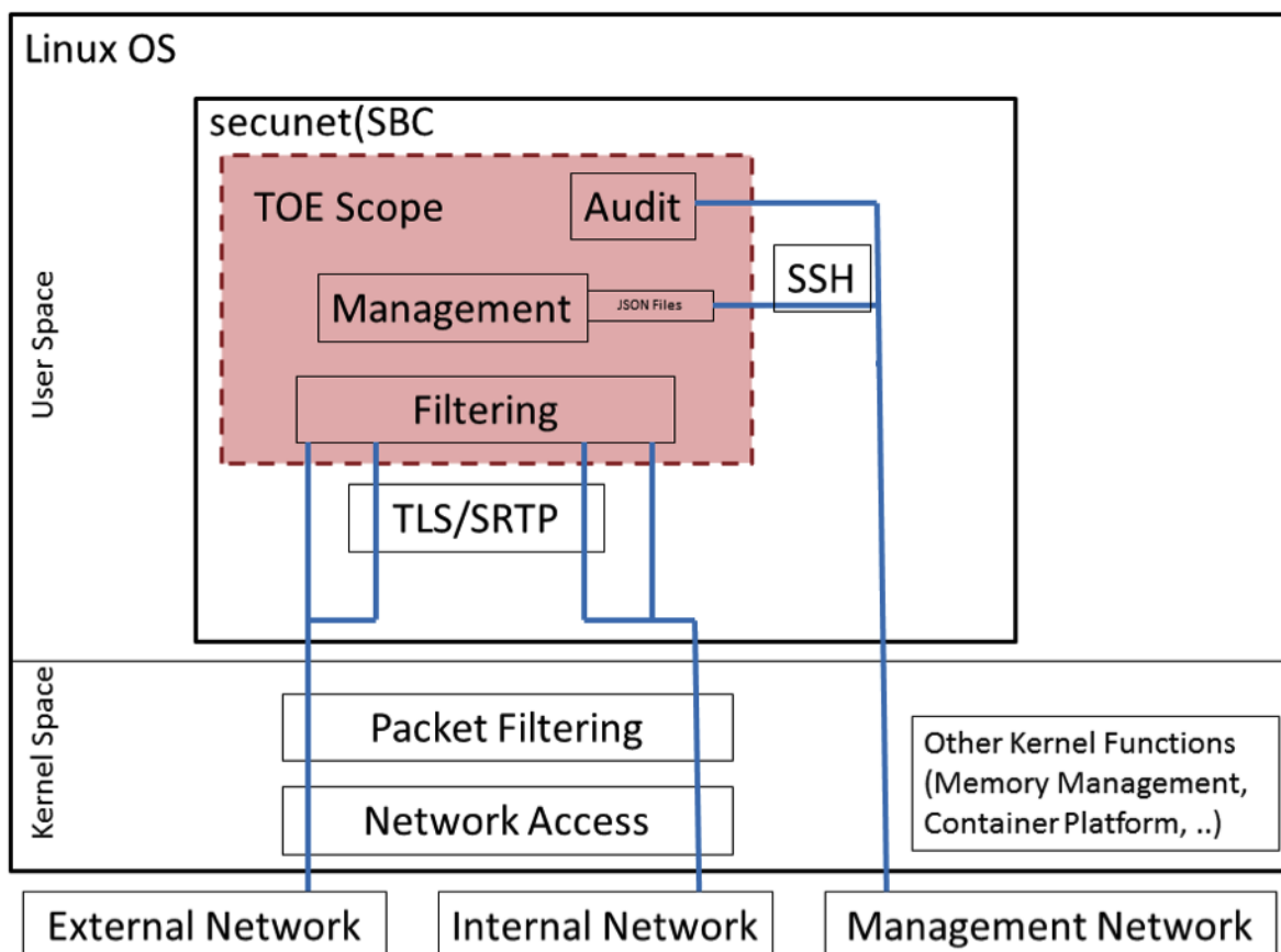
Figure 2: Logical TOE Scope
