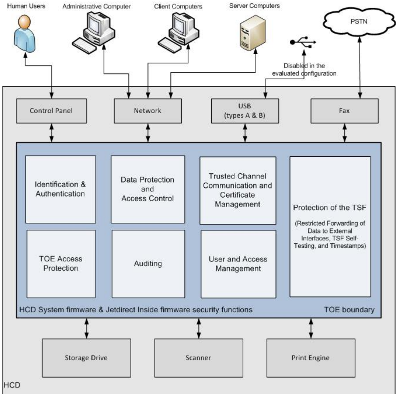
Figure 2: HCD logical diagram
