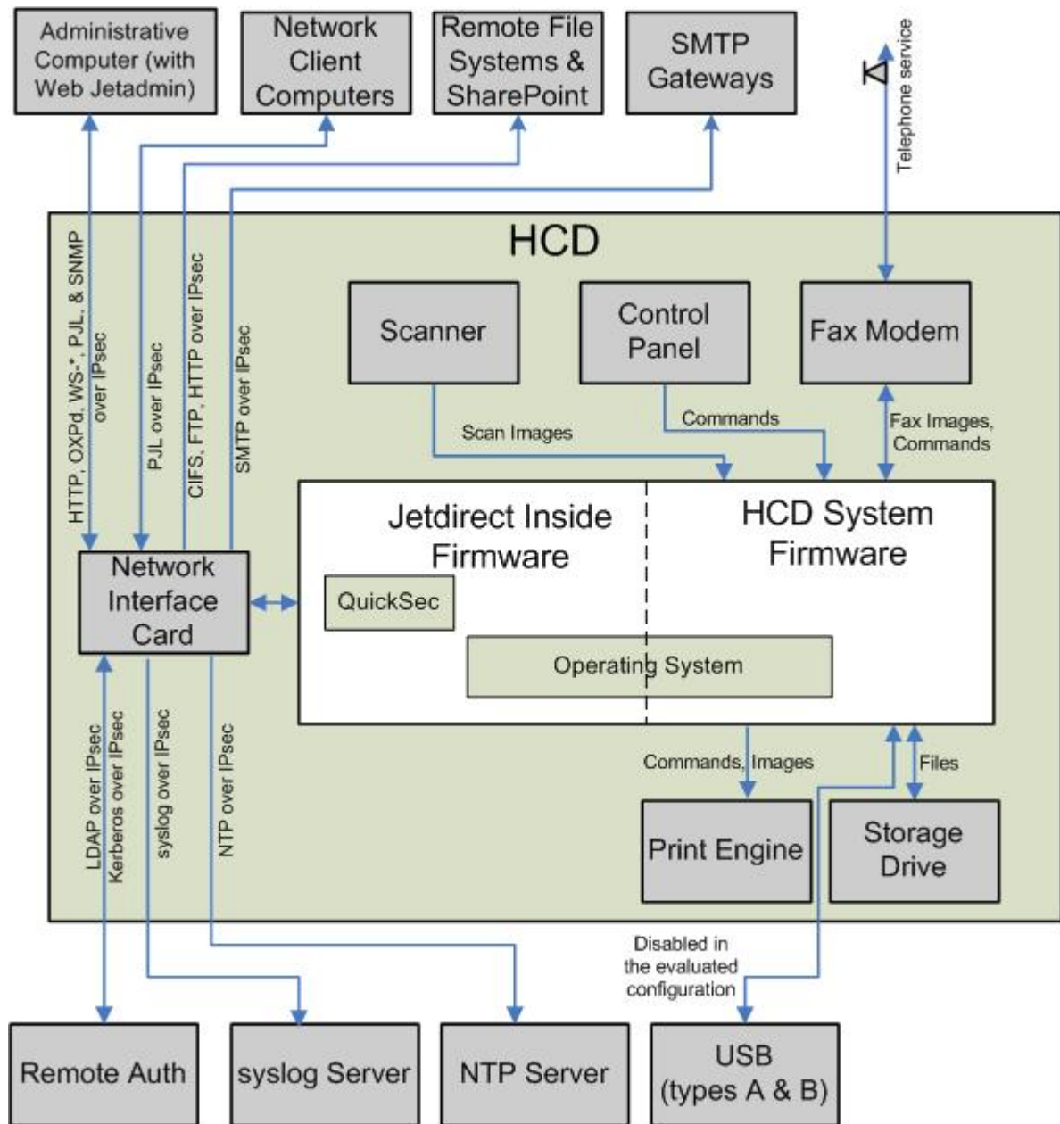
Figure 1: HCD physical diagram
