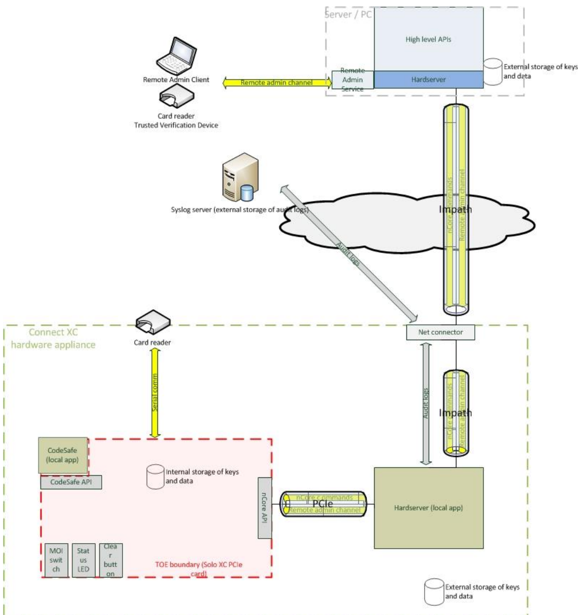
Figure 3 Configuration 1: TOE in Connect XC
