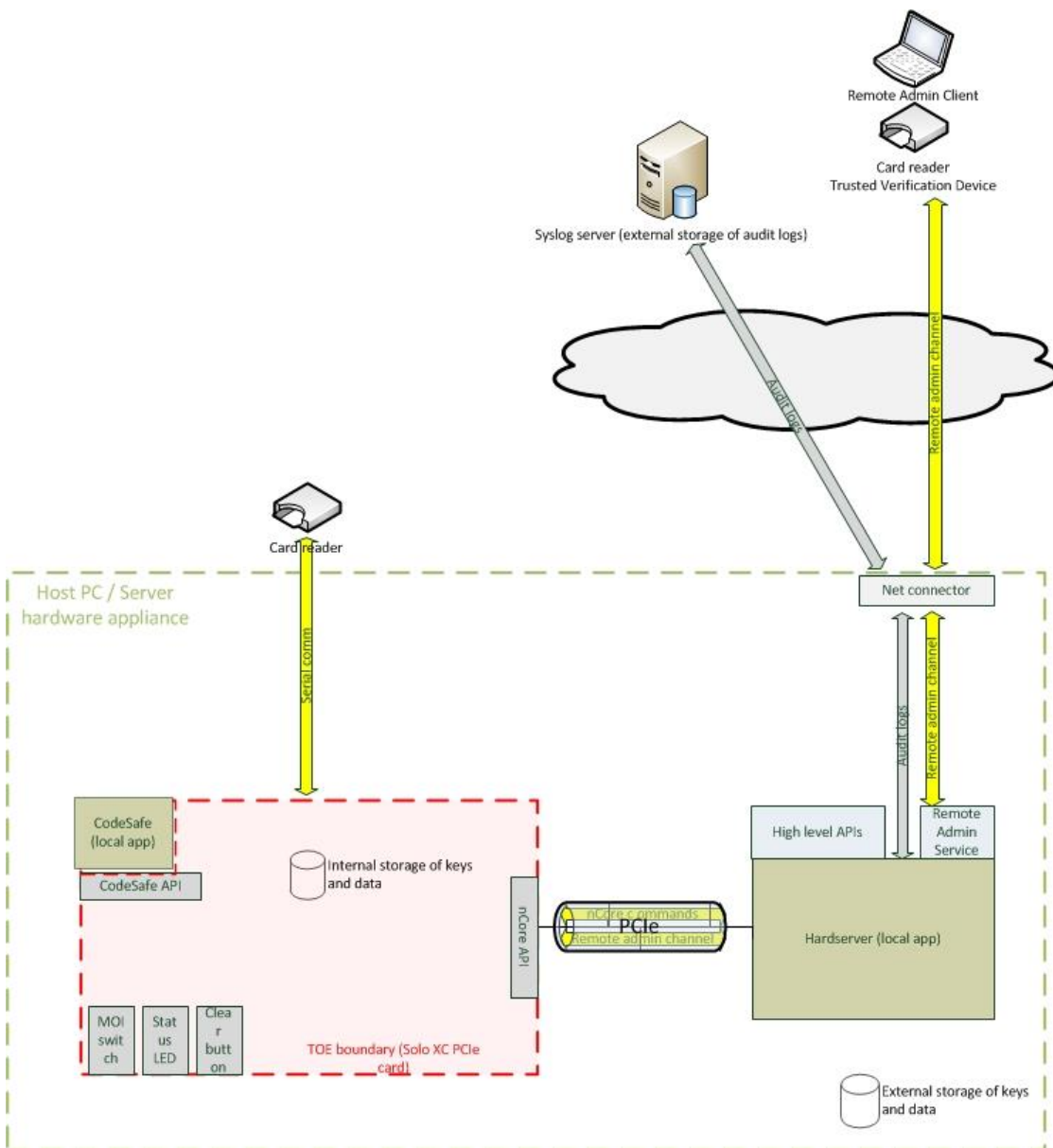
Figure 4 Configuration 2: TOE in host server
