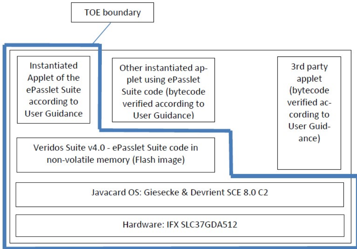
Figure 1 TOE components.
