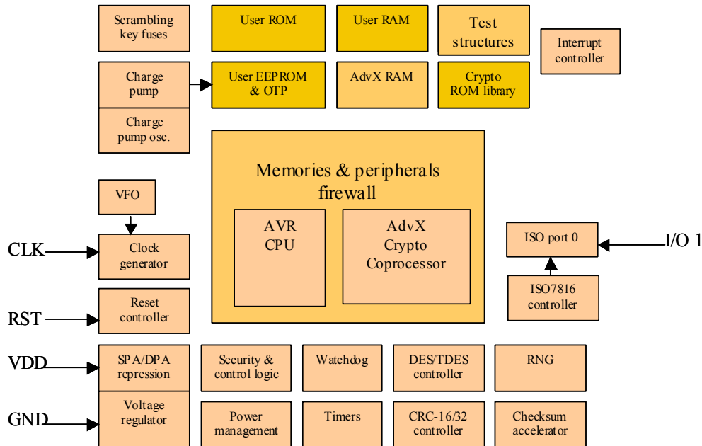
Figure 1 - micro-circuit ATMEL AT90SC12836RCT
