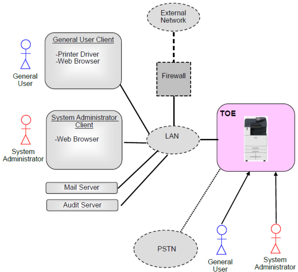
Figure 4-1 Operational Environment of the TOE (except when updating the firmware)
