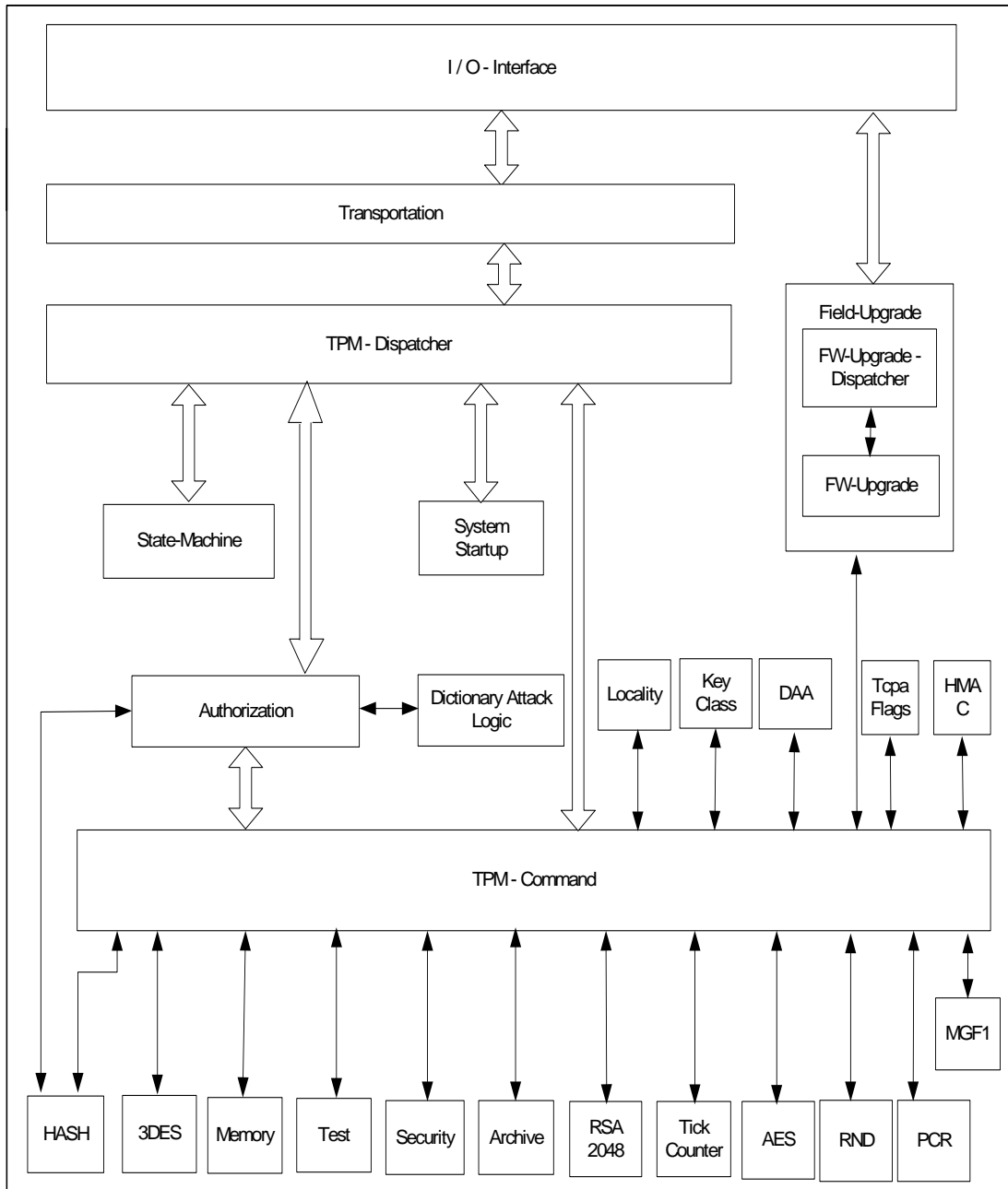
Figure 2: Firmware block diagram of the SLB9635TT1.2
