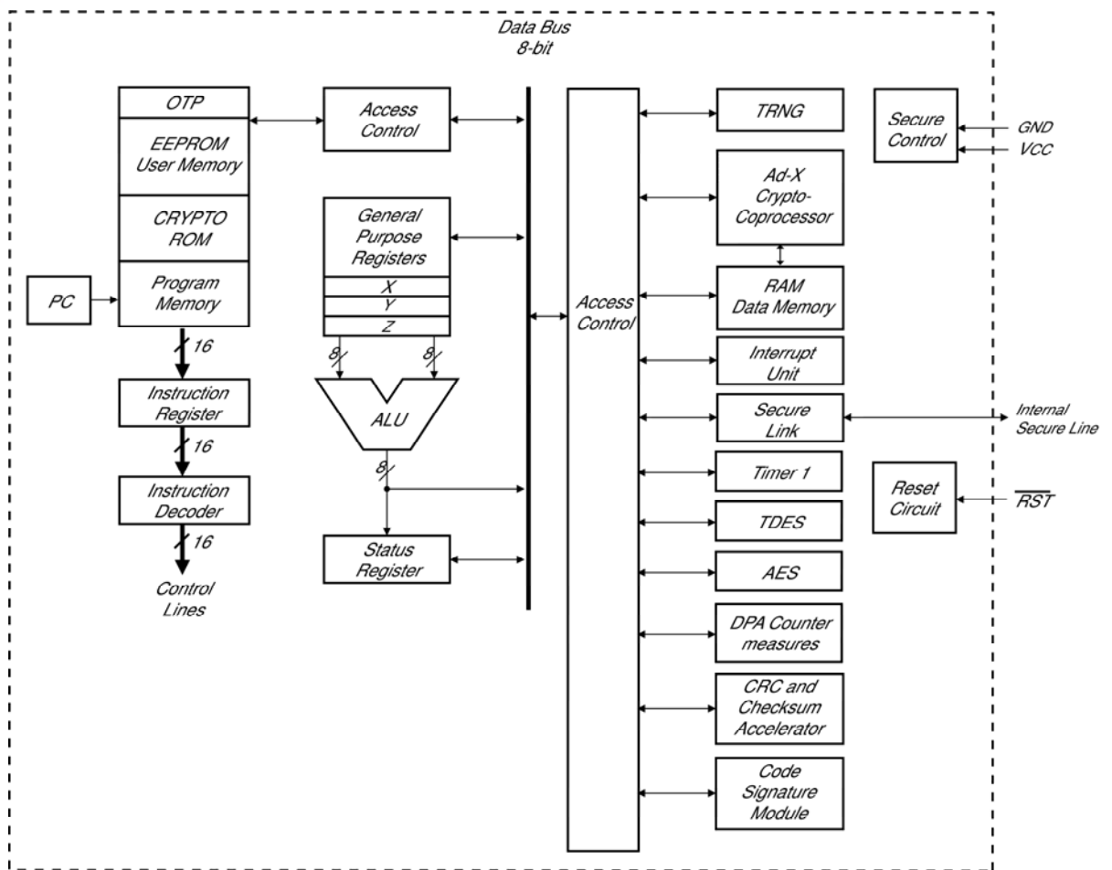
Figure 3: Block Diagram of the Secure Core
