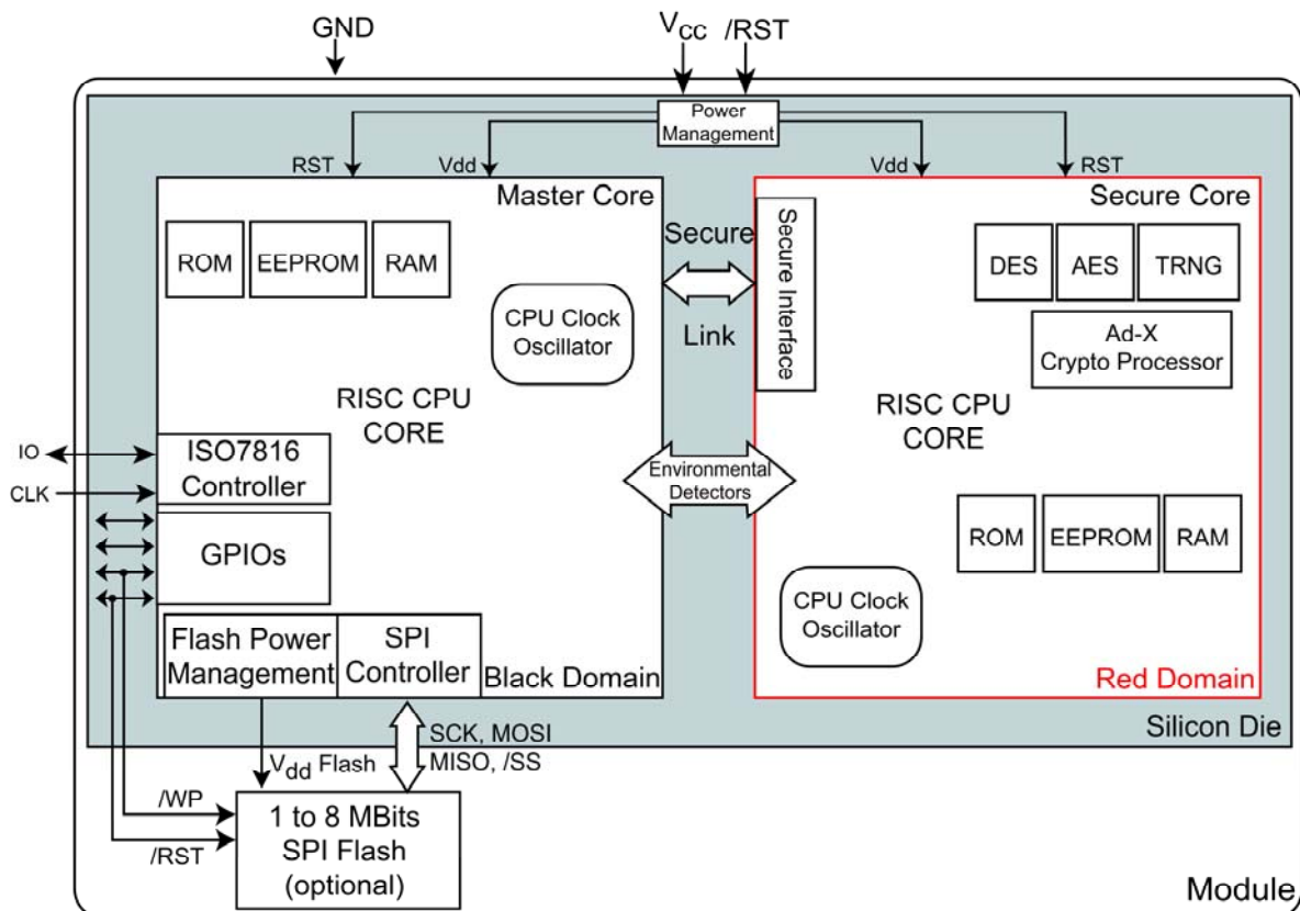
Figure 1: Overview of the 2 cores and how they are connected
