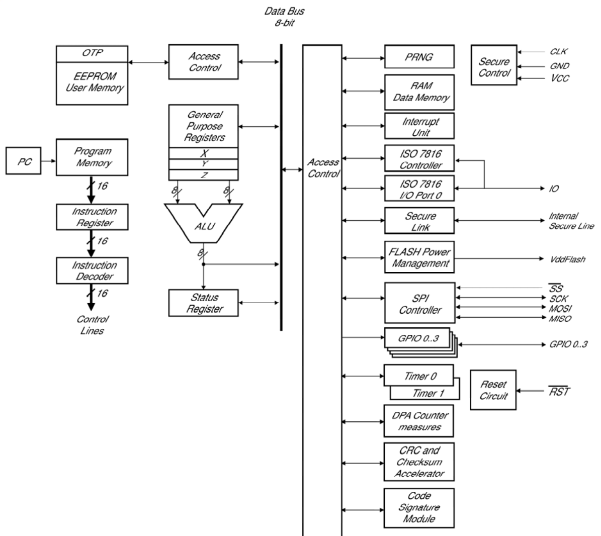
Figure 2: Block Diagram of the Master Core
