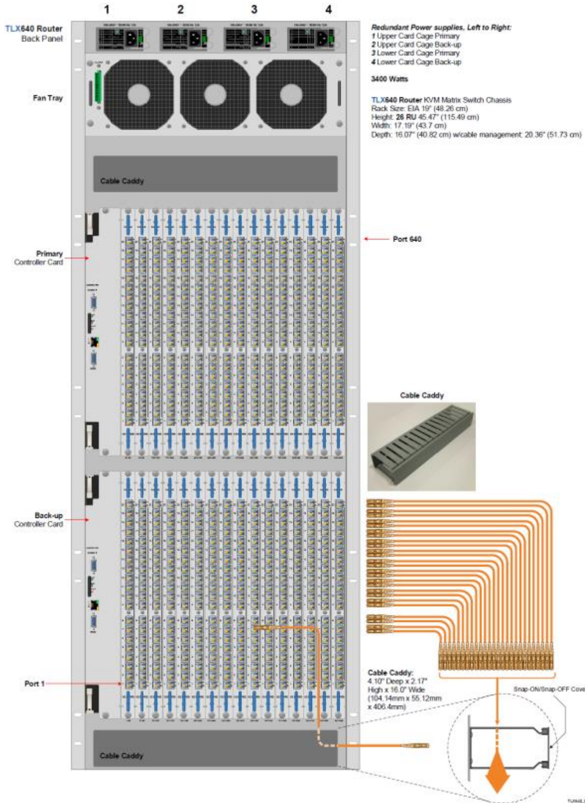
Figure 1a. Thinklogical TLX640 Matrix Switch
