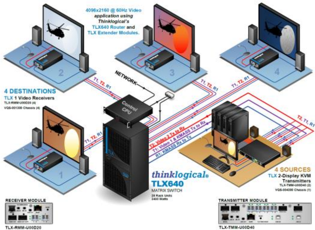
Figure 2a. Typical TOE TLX640 Configuration
