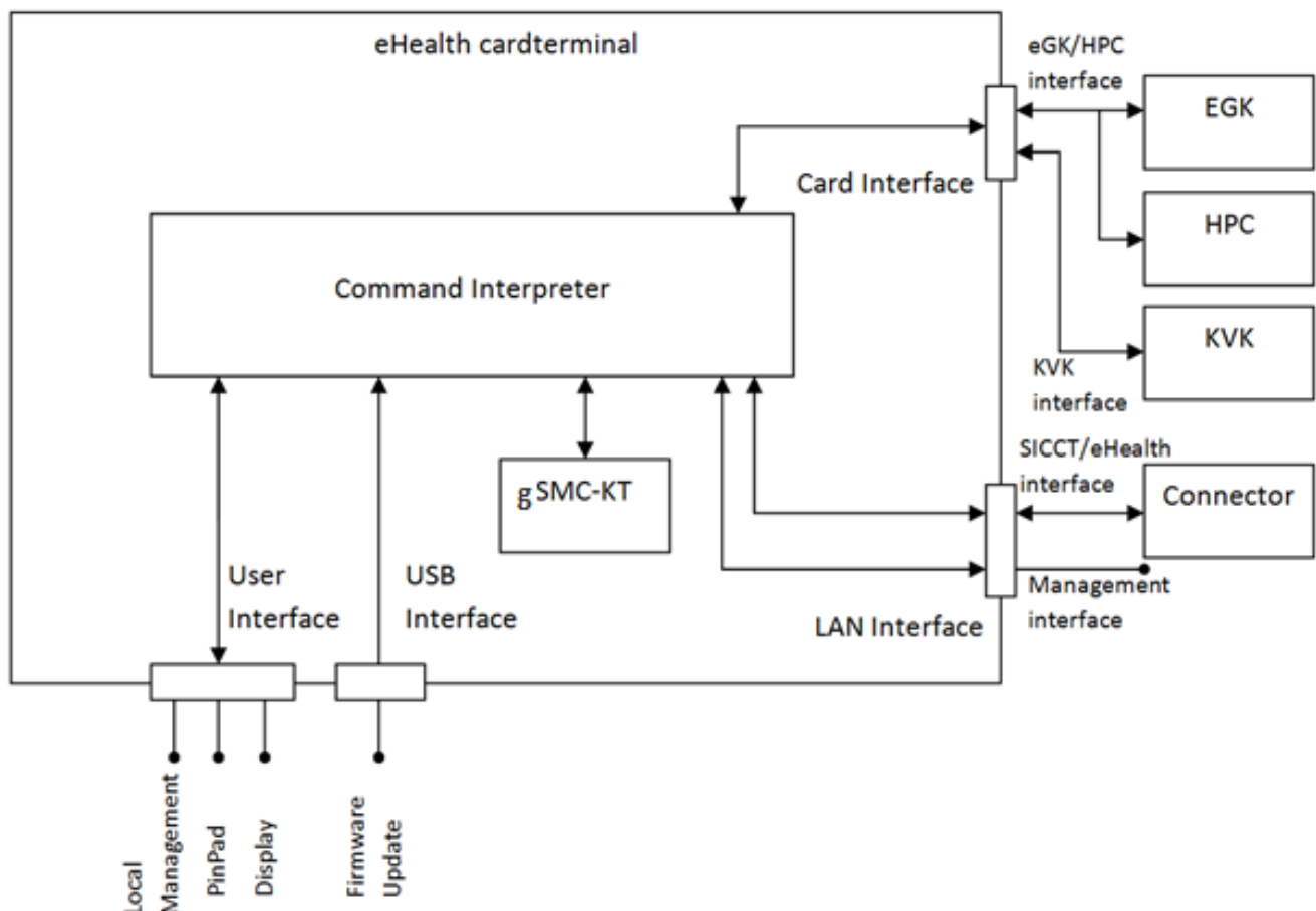
Figure 1: TOE architecture (logical perspective)
