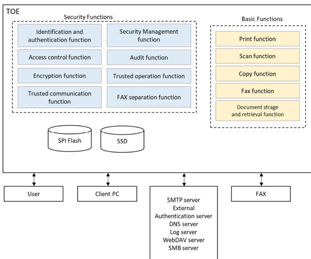
Figure 1-2 The logical scope of TOE
