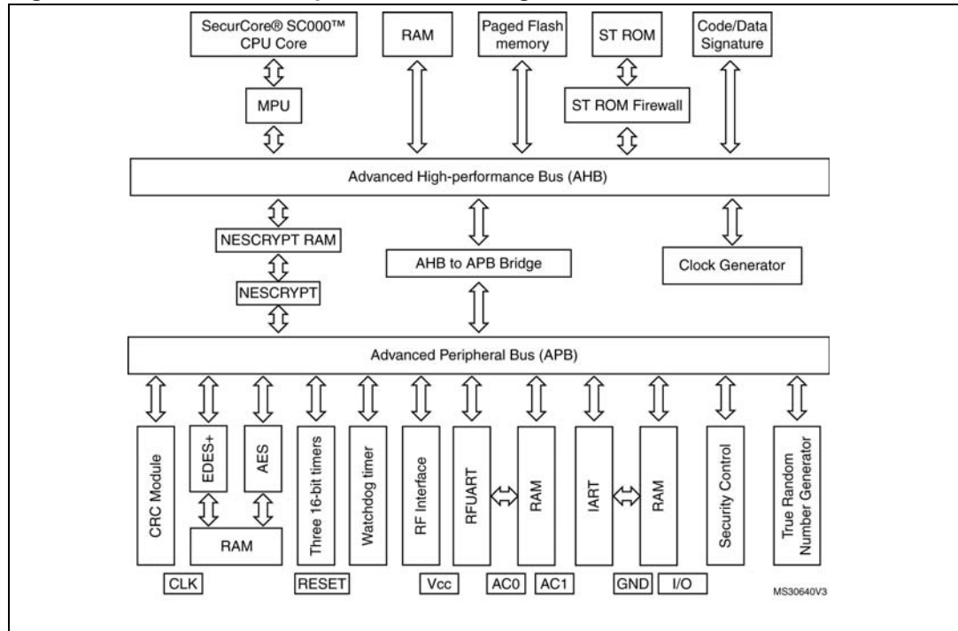
Figure 1. ST31G480 G01 platform block diagram
