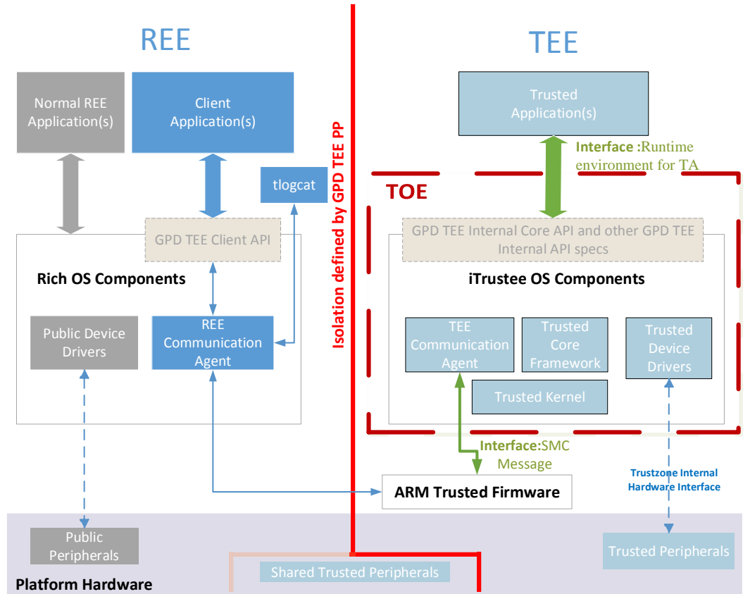
Figure 1: The architecture of a TOE-enabled device
