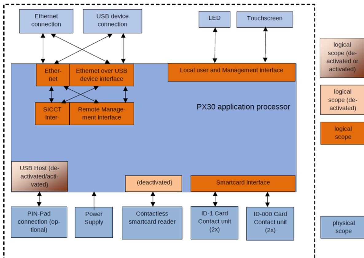
Figure 1: TOE Architecture
