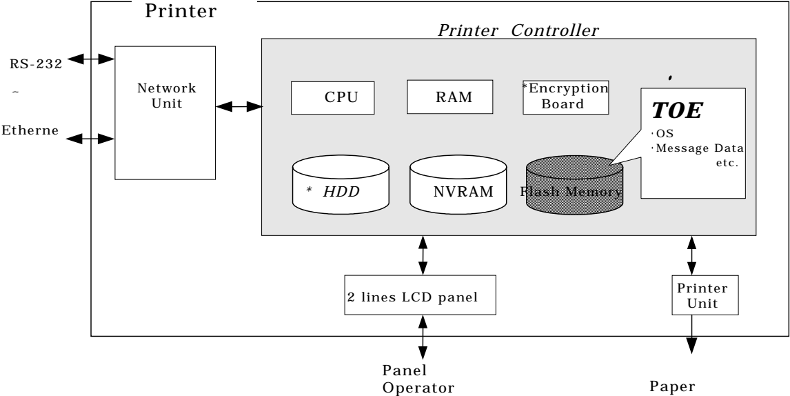
Figure 2-1 Configuration of Developer Testing
