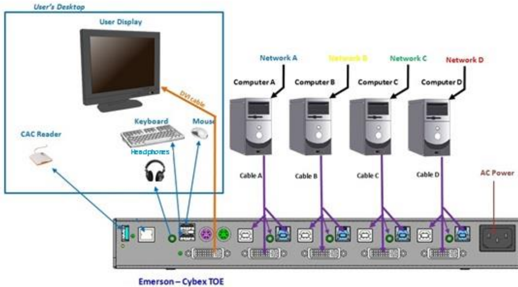
Figure 1: Typical example of a secure KVM TOE installation
