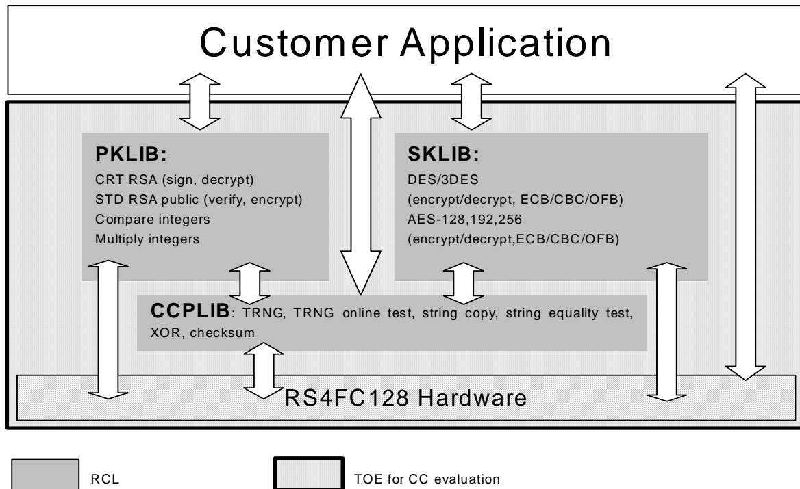
Figure 1-2: RCL3.0 (TOE Software), TOE Hardware and Customer Application
