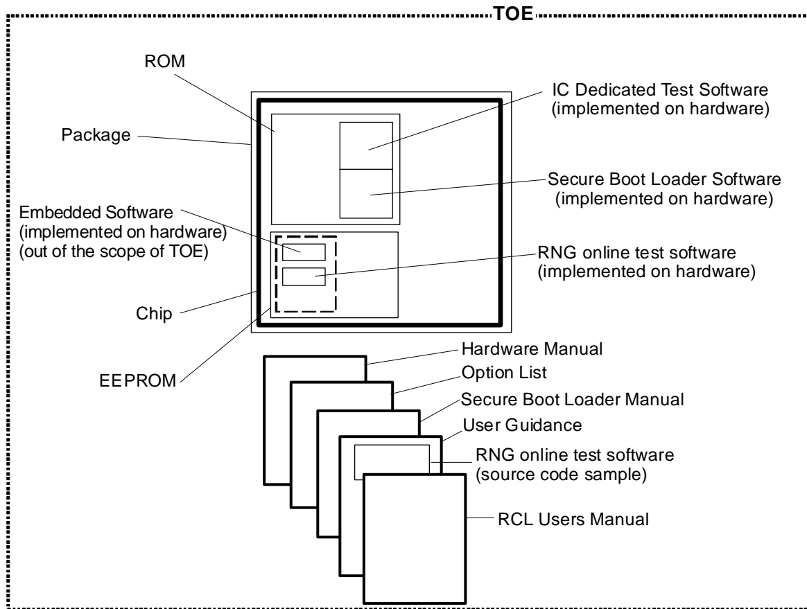
Figure 1-1: Configuration of the TOE
