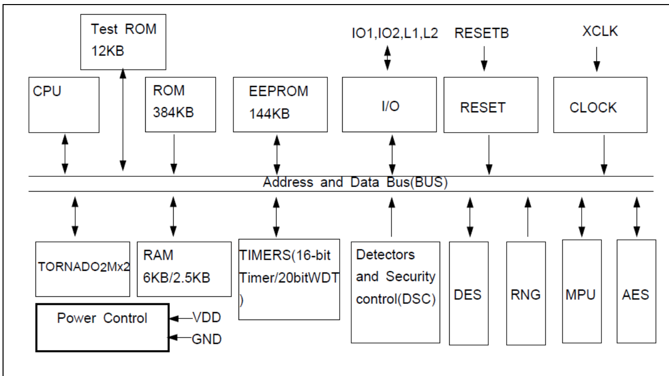
Figure 1. S3CT9KW Block Diagram
