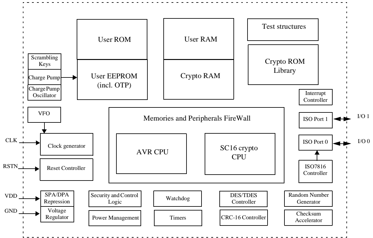
Fig. 2.1 -VEGA2 AT90SC19264RC Block Diagram
