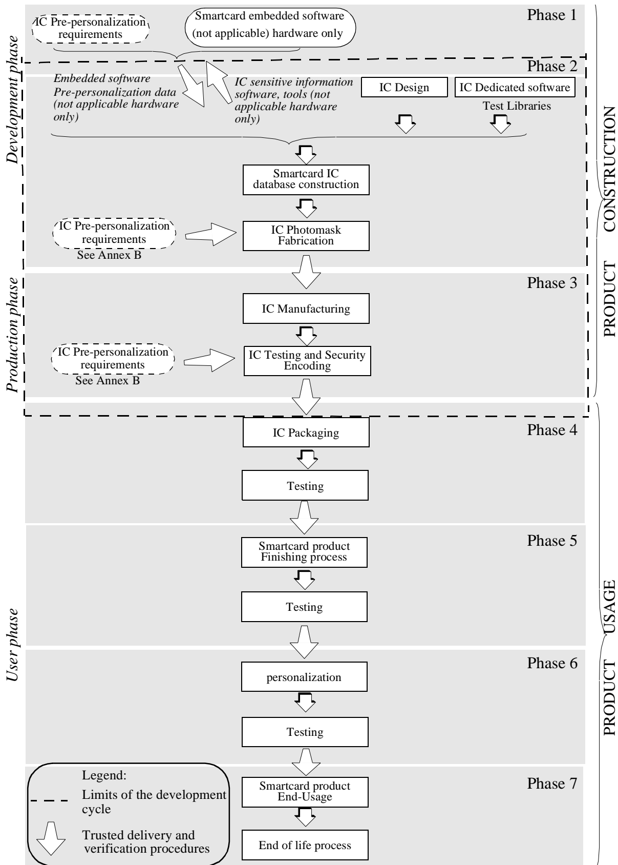
Fig. 2.2 -The Smartcard Product Life Cycle
