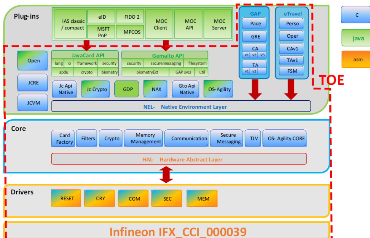
Figure 1: TOE Boundaries
