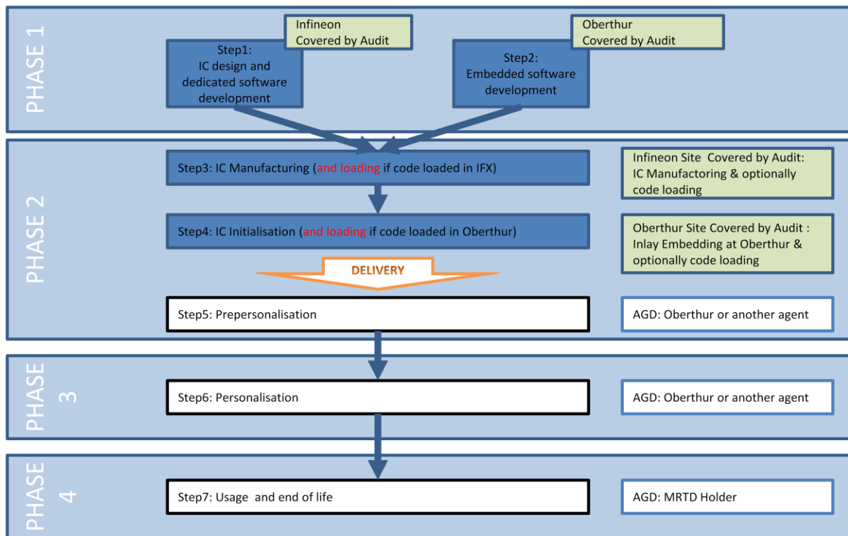
Figure 2: ePass ICAO Essential life cycle
