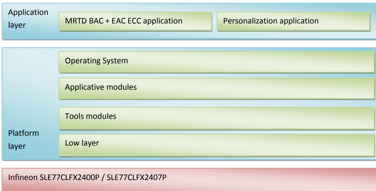
Figure 1 - TOE architecture
