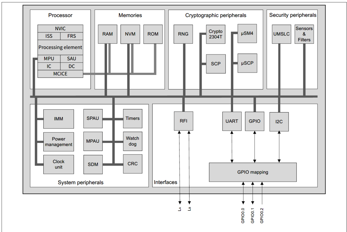
Figure 1 TOE hardware
