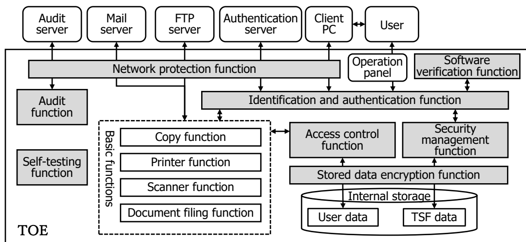
Figure 5-1 TOE boundary
