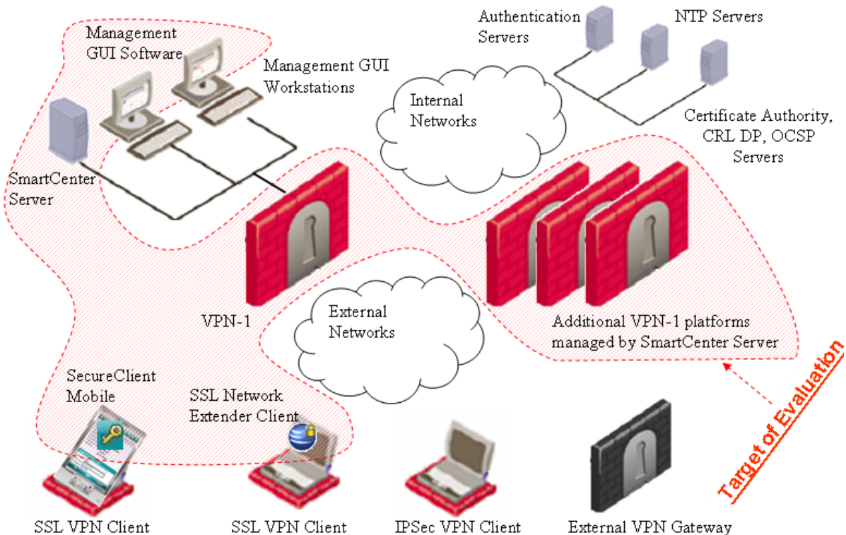
Figure 2 - TOE Architecture
