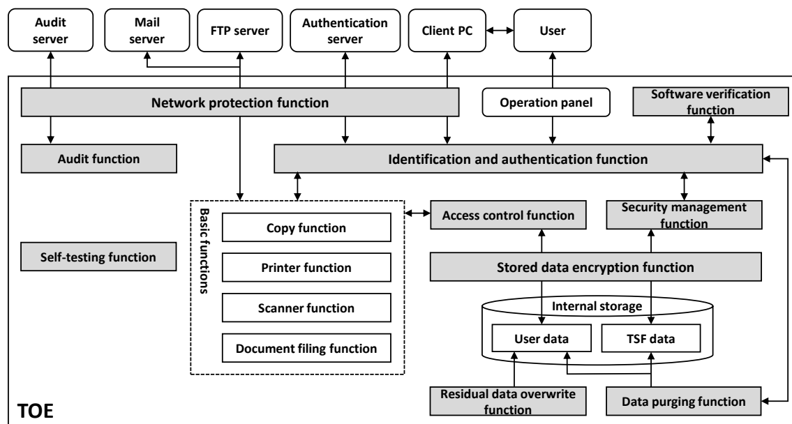
Figure 5-1 TOE boundary
