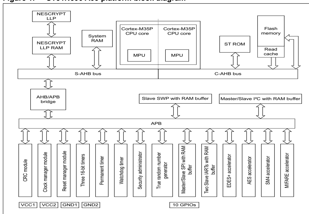
Figure 1. ST31N600 A03 platform block diagram
