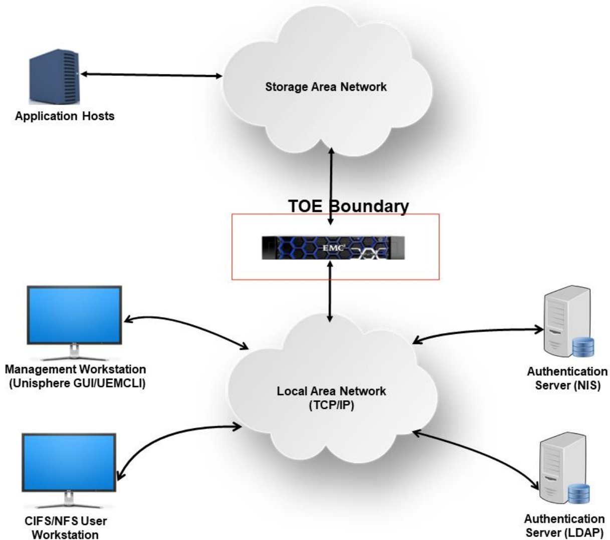
Figure 1: TOE Architecture
