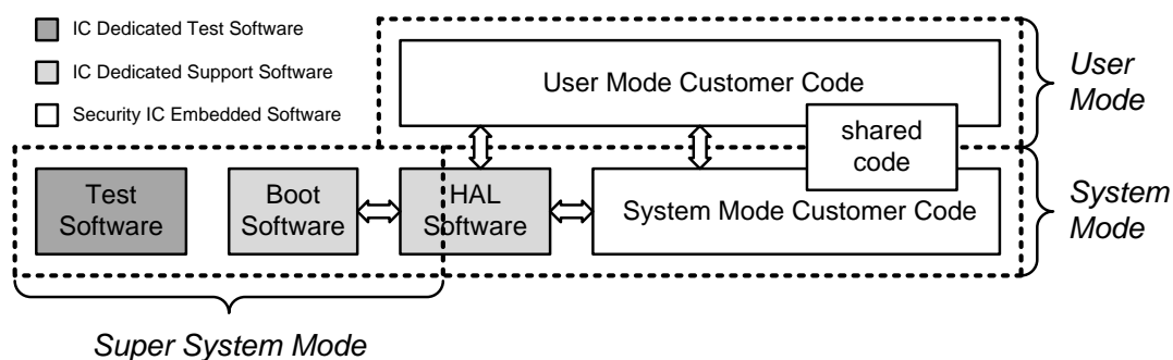
Fig. 1.2: Software Components of the TOE
