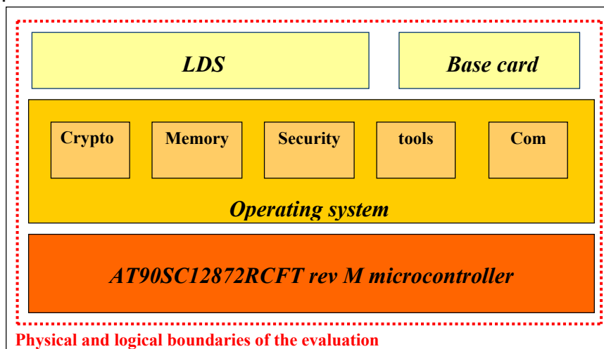
Figure 1 – Product architecture
