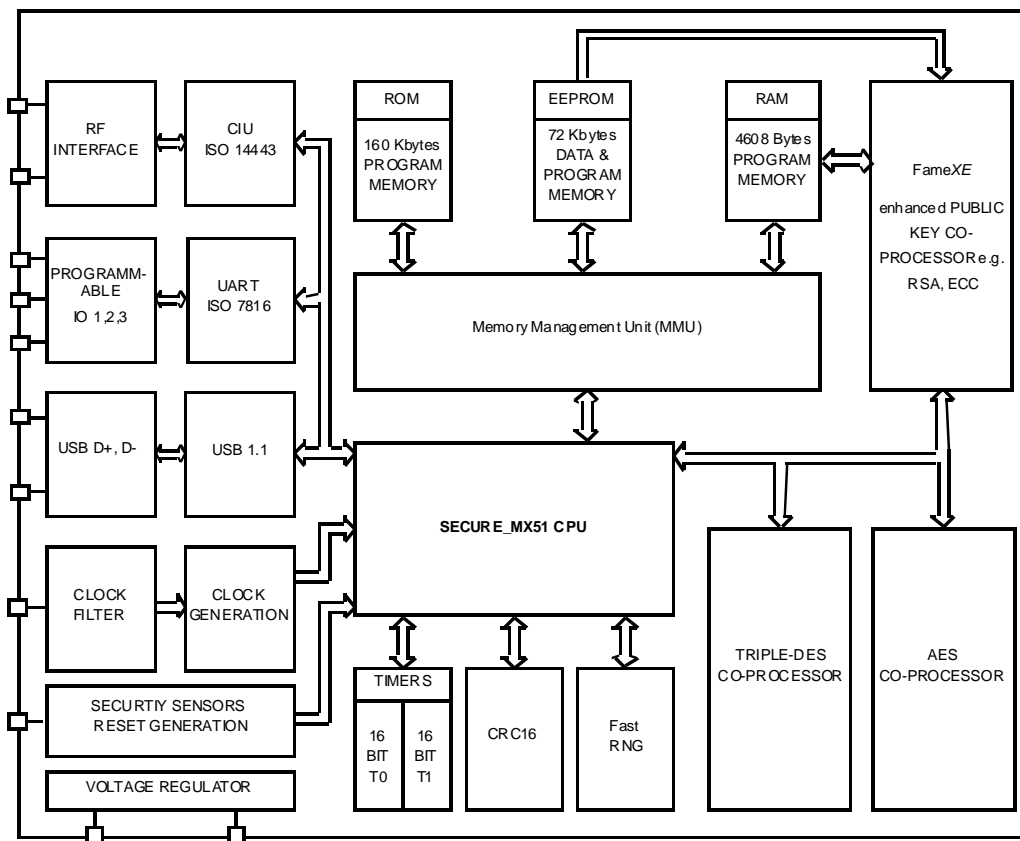
Figure 1: Block Diagram of the P5CT072V0P
