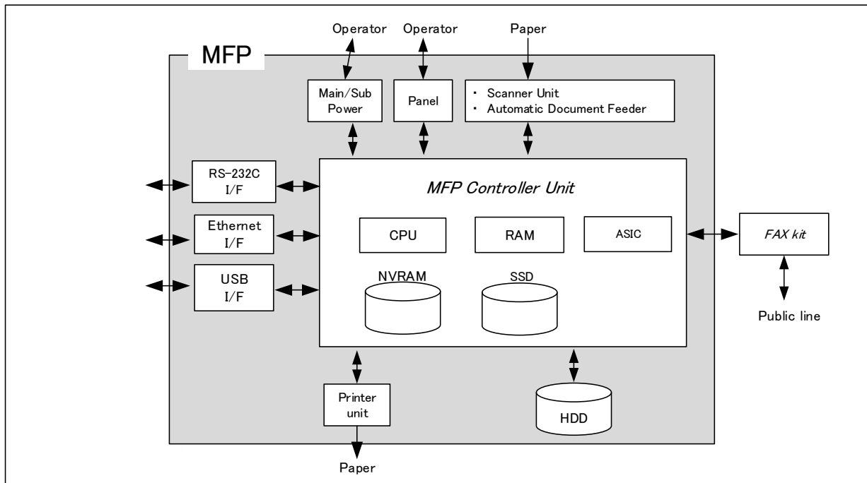
Figure 1-2 Physical scope of the TOE
